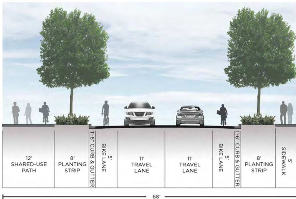
Figure 2: Proposed Typical Street Cross-Section
