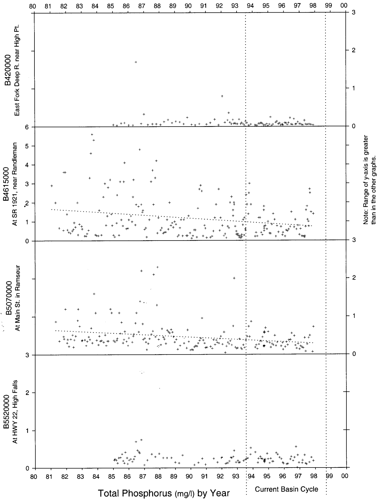
Figure A-37. Measurements of total phosphorus (y-axis) over time (x-axis) from four monitoring stations along the Deep River. (Stations are arranged in an upstream (top) - downstream (bottom) pattern.)
