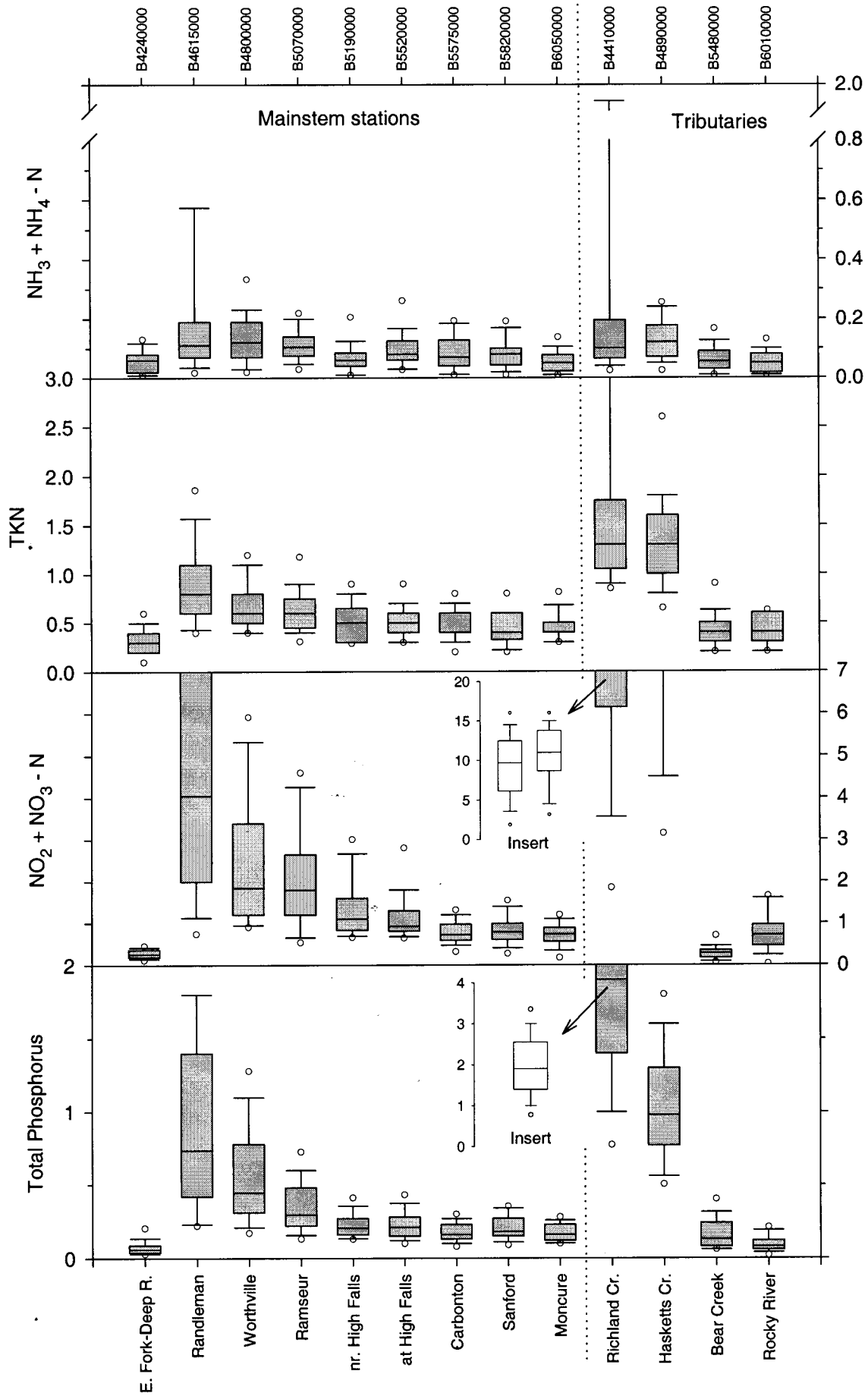
Figure A-7. Nutrients (mg/l) for the Deep R. mainstem and tributaries (1993-1997). (Inserts represent exanded views of adjacent plots)
