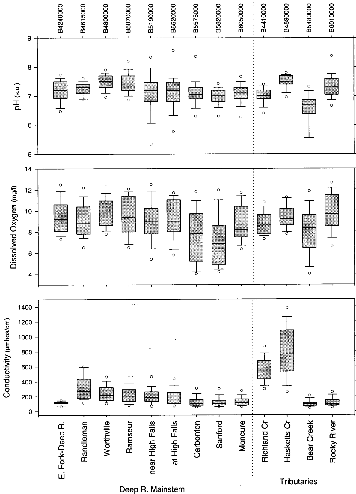
Figure A-6. Box plots for dissolved oxygen, pH and conductivity for the monitoring stations along the mainstem and tributaries of the Deep River (1993-1997).
