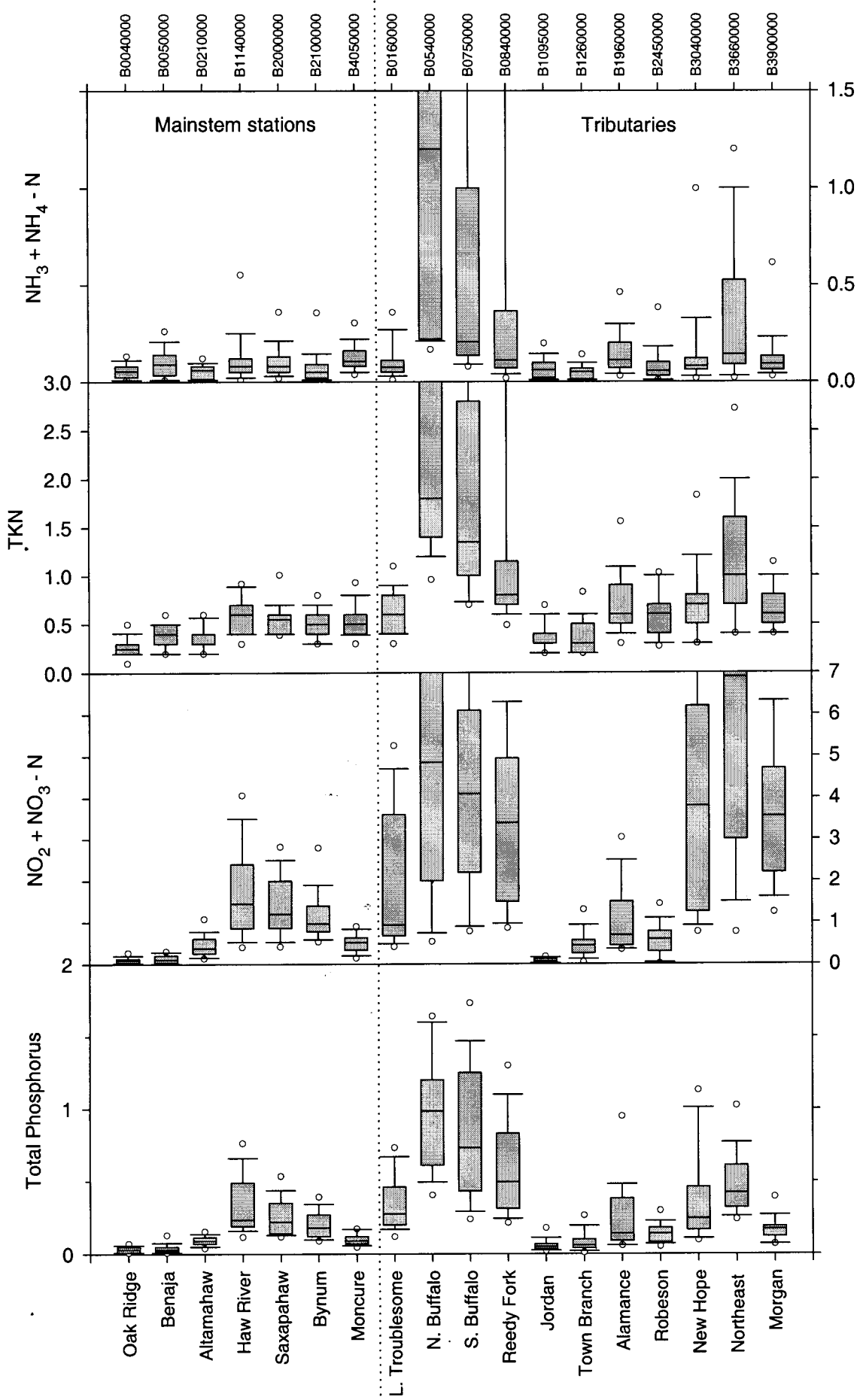
Figure A-5. Nutrients (mg/l) for the Haw R. mainstem and tributaries (1993-1997).
