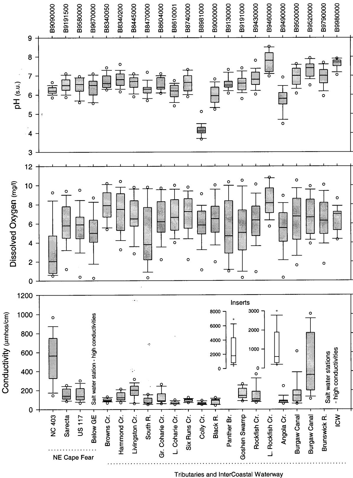
Figure A-46. Box plots for dissolved oxygen, pH and conductivity for the monitoring stations along tributaries of the Cape Fear River (1996-1998). (Data were collected by the Lower Cape Fear River Program.)
