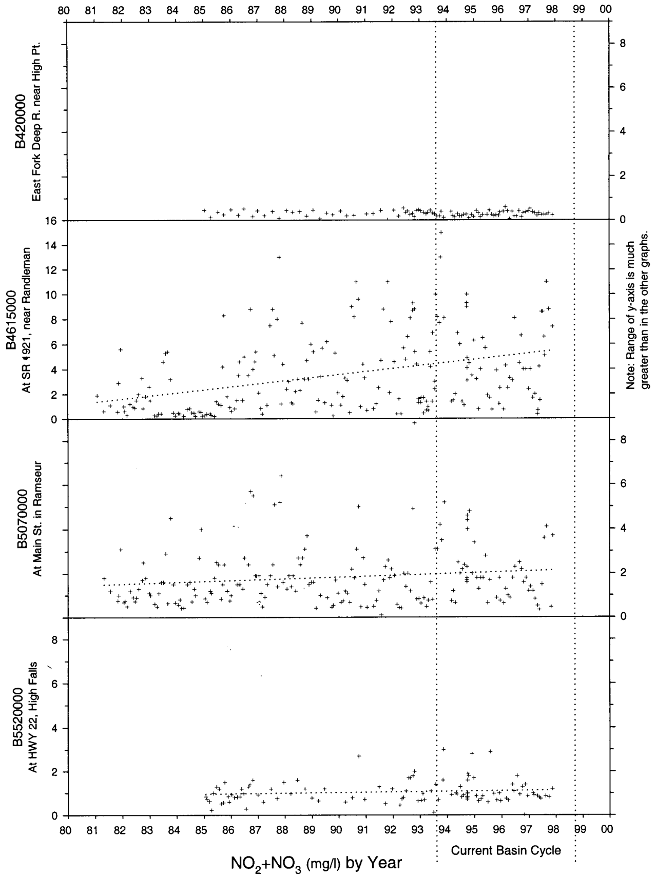
Figure A-36. Measurements of nitrite+nitrate-nitrogen (y-axis) over time (x-axis) from four monitoring stations along the Deep River. (Stations are arranged in an upstream (top) - downstream (bottom) pattern.)
