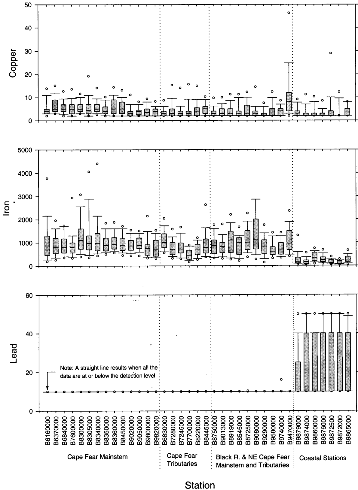
Figure A-21. Box plots of the concentrations ( \mu\text{g/l} ) of copper, iron and lead for the monitoring stations along Cape Fear, Black, NE Cape Fear rivers, and along the coast.
