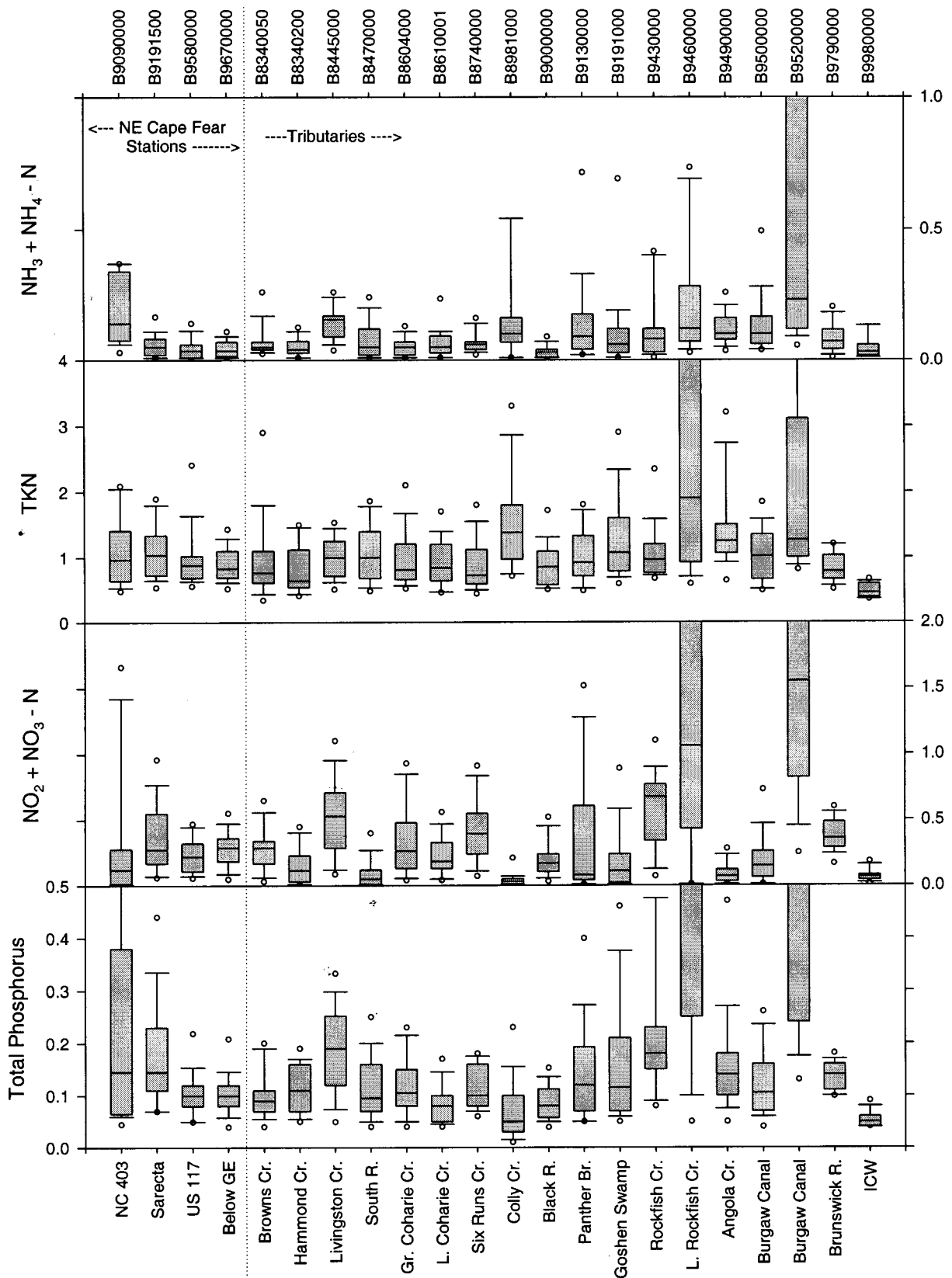
Figure -48. Box plots for nutrients (mg/l) for the monitoring stations along the tributaries of the Cape Fear River. (Data were collected by the Lower Cape Fear River Program)
