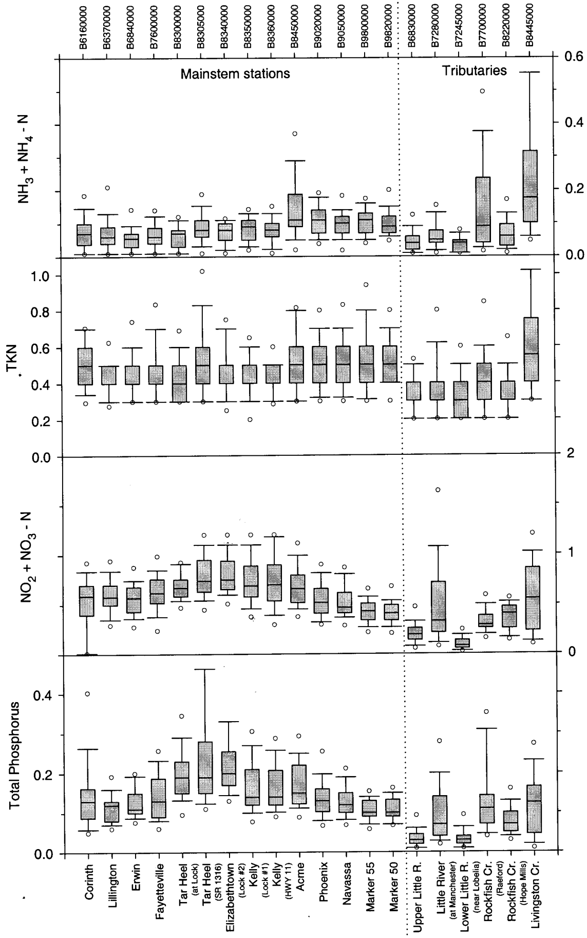
Figure A-9. Nutrients (mg/l) for the Cape Fear R. mainstem and tributaries (1993-1997).
