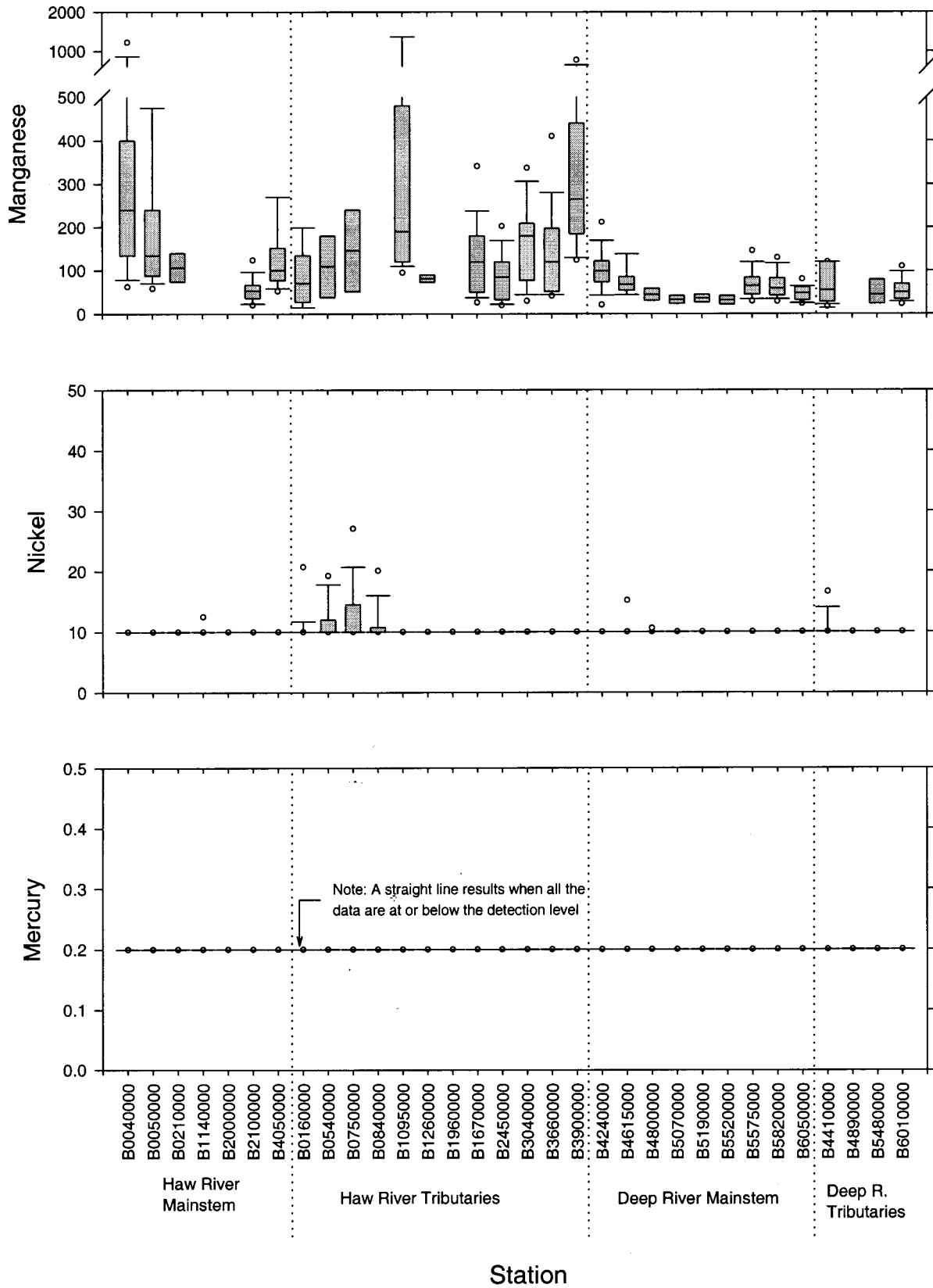
Figure A-22. Box plots of the concentrations ( \mu\text{g/l} ) of manganese, nickel and mercury for monitoring stations along the Haw and Deep rivers.
