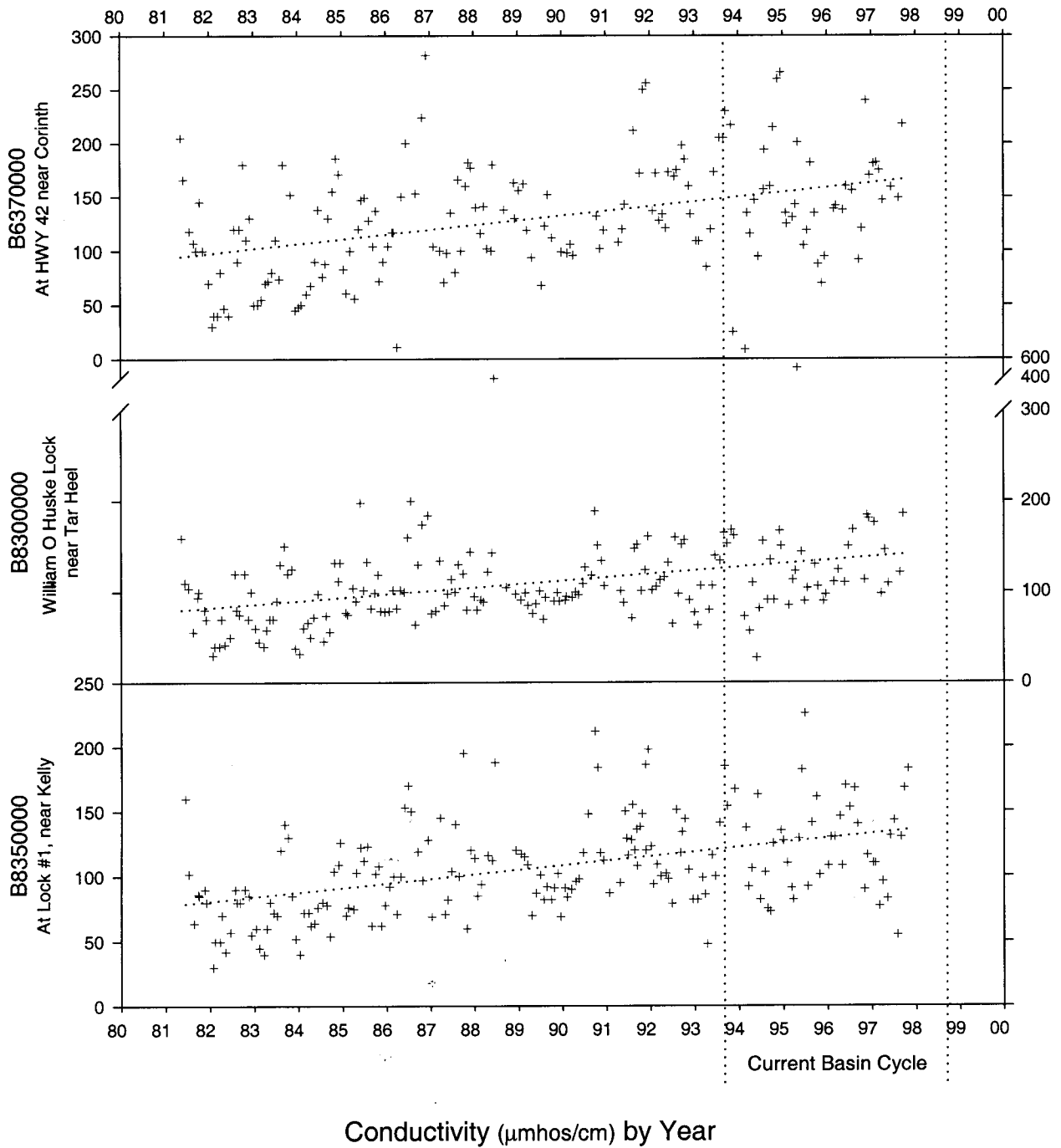
Figure A-39. Measurements of conductivity (y-axis) over time (x-axis) from three monitoring stations along the Cape Fear River. (Stations are arranged in an upstream (top) - downstream (bottom) pattern.)
