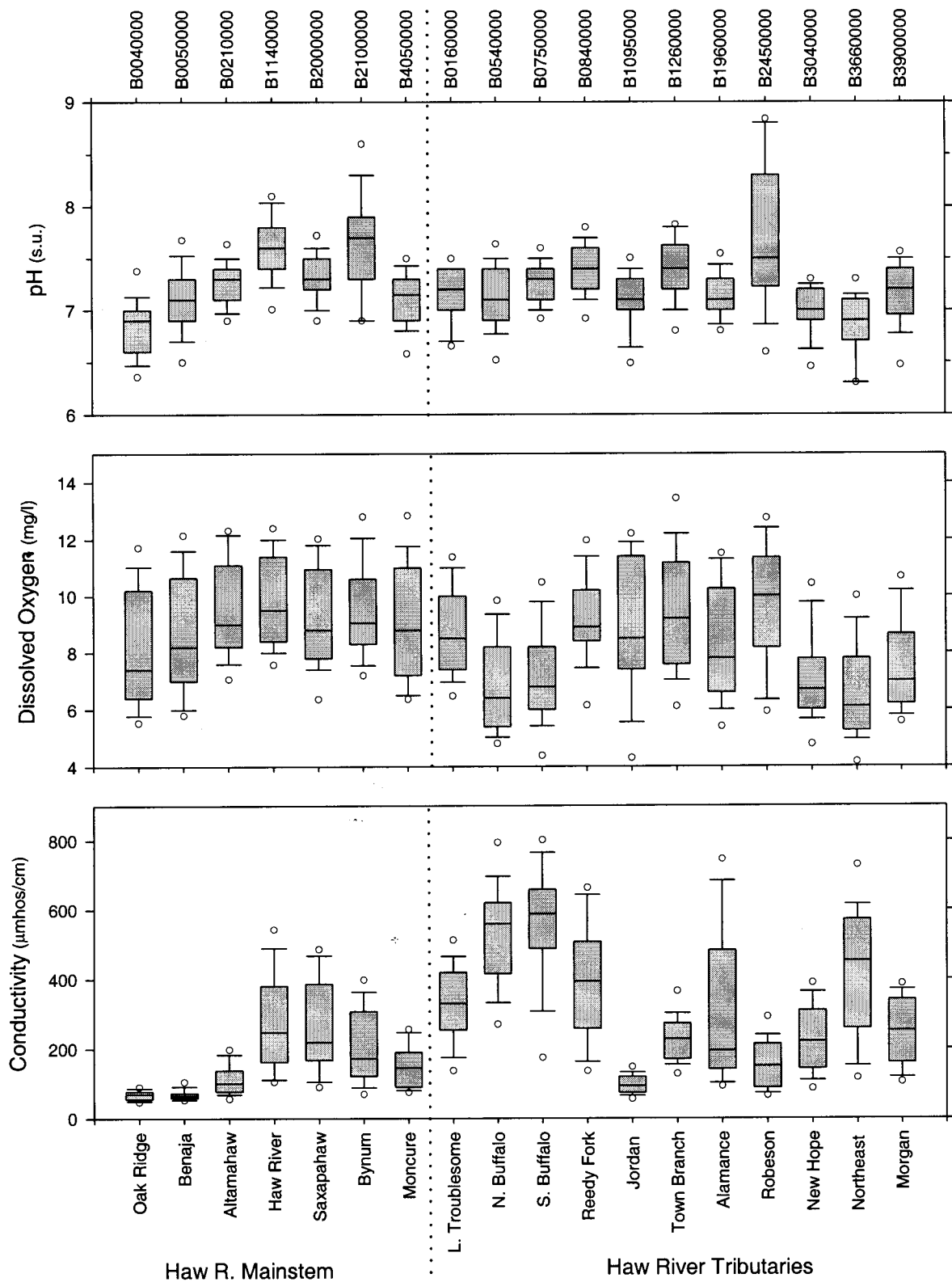
Figure A-4. Box plots for dissolved oxygen, pH and conductivity for the monitoring stations along the mainstem and tributaries of the Haw River (1993-1997).
