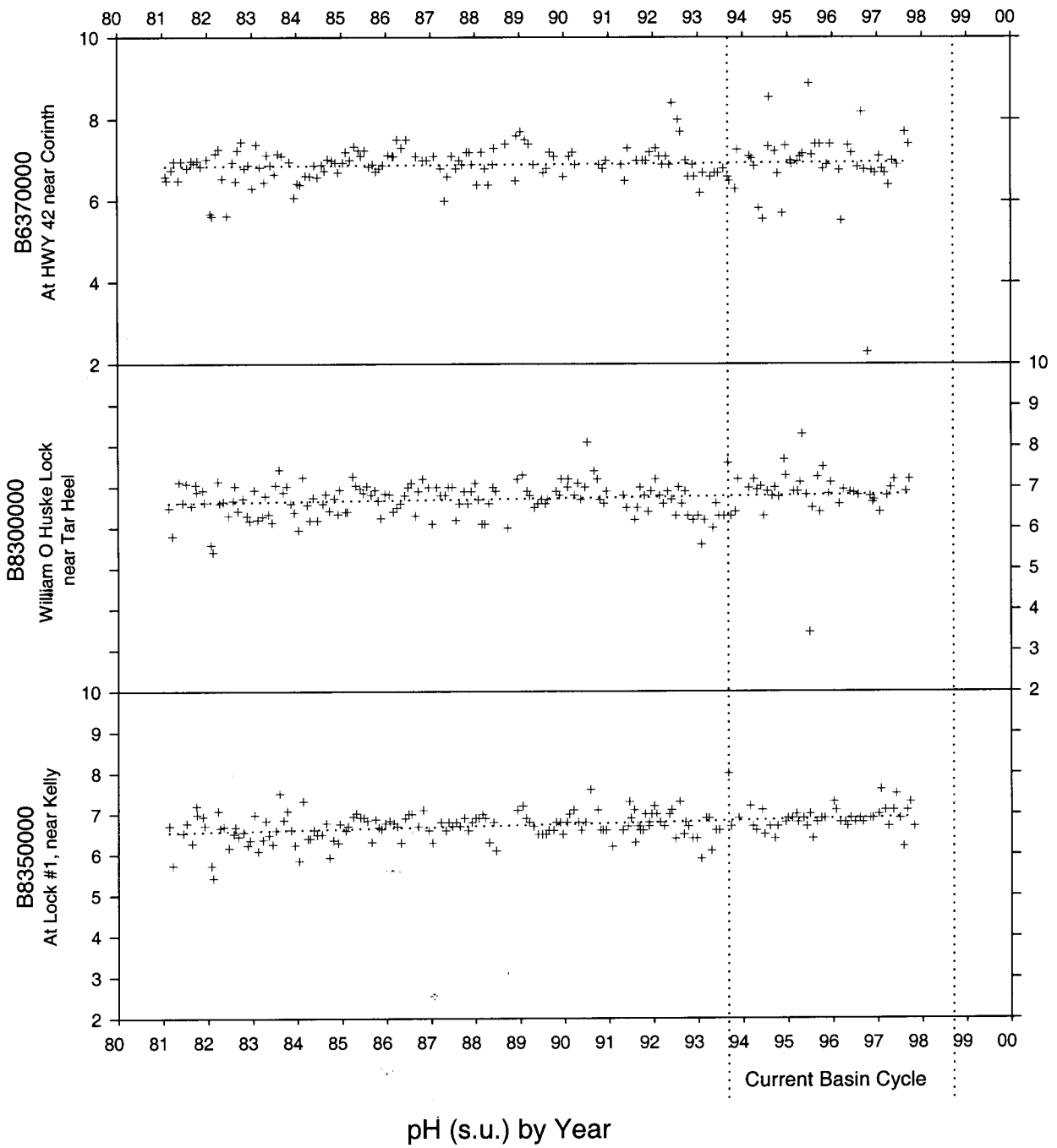
Figure A-38. Measurements of pH (y-axis) over time (x-axis) from three monitoring stations along the Cape Fear River. (Stations are arranged in an upstream (top) - downstream (bottom) pattern.)
