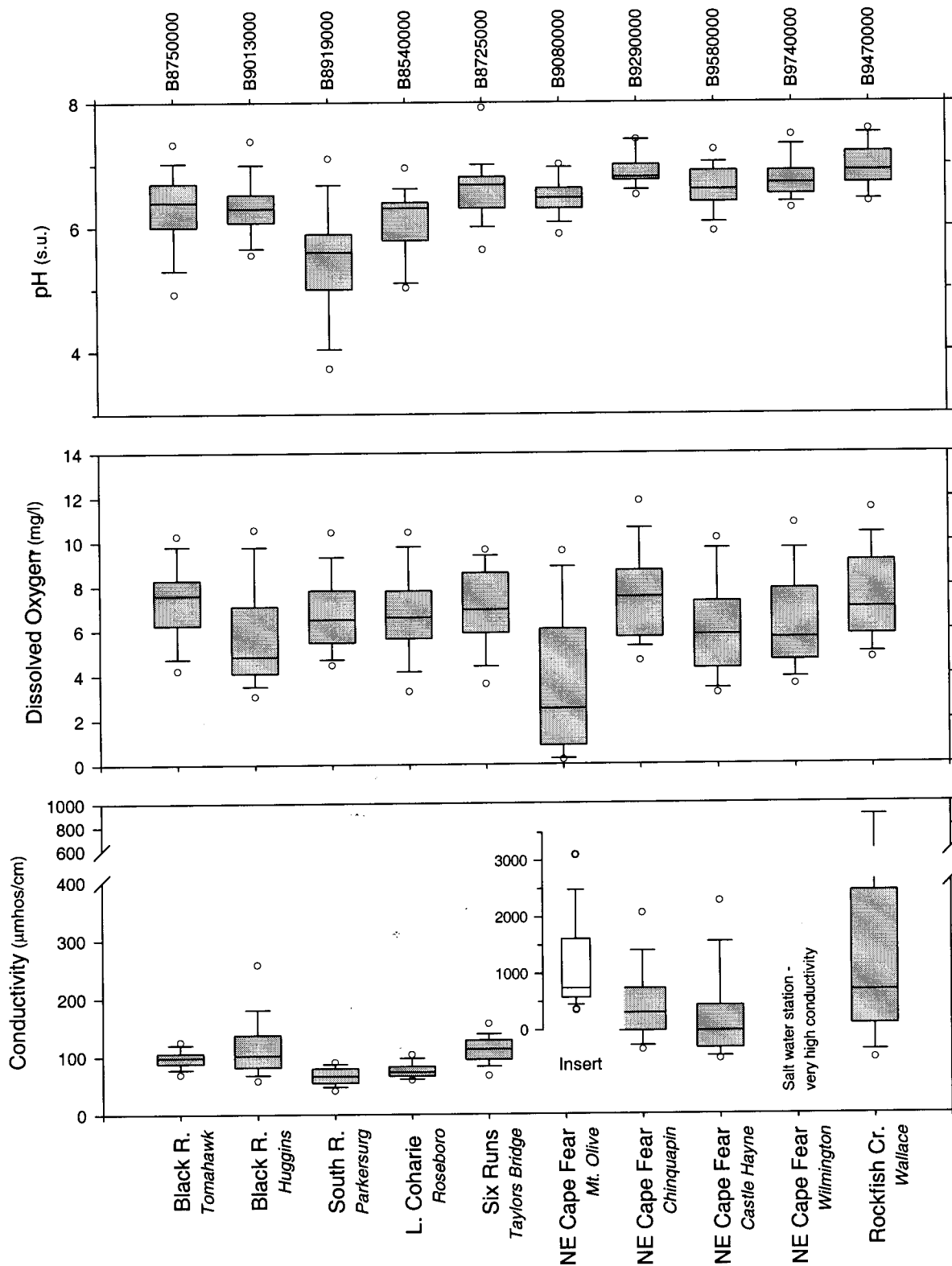
Figure A-10. Box plots for dissolved oxygen, pH and conductivity for the monitoring stations along the Black, South, NE Cape Fear Rivers and various tributaries (1993-1997). Figure 12 provides the temporal patterns of these parameters for station B9080000 near Mt. Olive.
