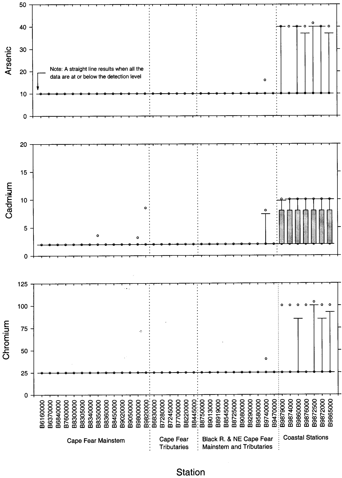
Figure A-19. Box plots of the concentrations (µg/l) of arsenic, cadmium and chromium for monitoring stations along the Cape Fear, Black, NE Cape Fear rivers and along the coast.
