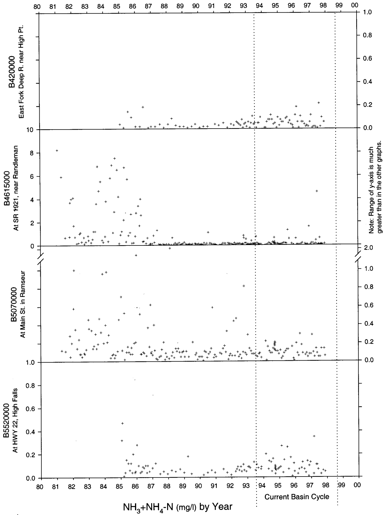
Figure A-34. Measurements of ammonia nitrogen (y-axis) over time (x-axis) from four monitoring stations along the Deep River. (Stations are arranged in an upstream (top) - downstream (bottom) pattern.)
