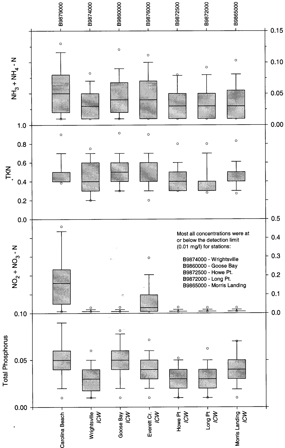
Figure A-15. Nutrients (mg/l) for the coastal stations (1993-1997).
