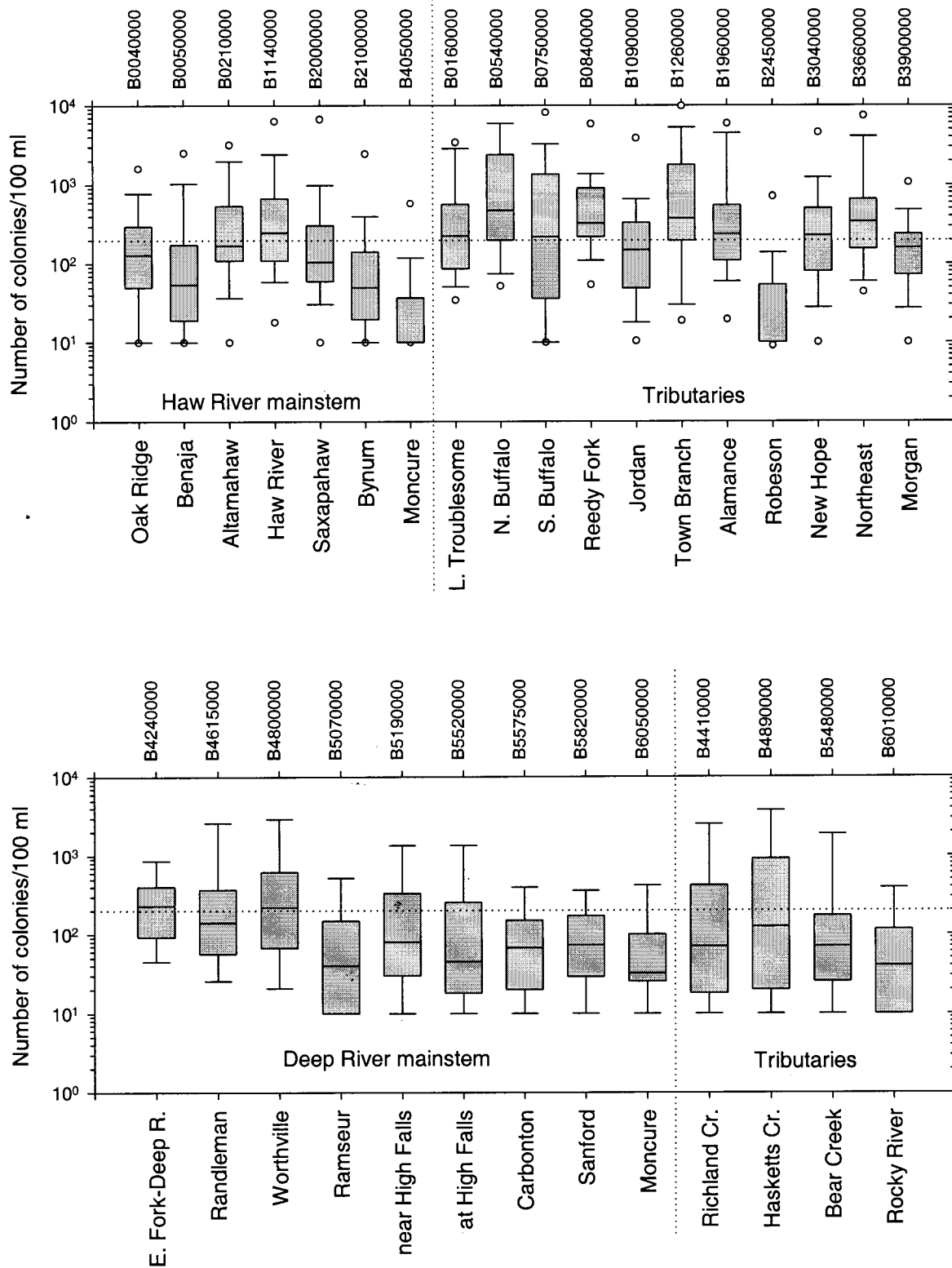
Figure A-16. Concentrations of fecal coliform bacteria 1993-1997. (Note the logarithmic scaling for the y-axis. A reference line representing 200 colonies per 100 milliliters is provided.)
