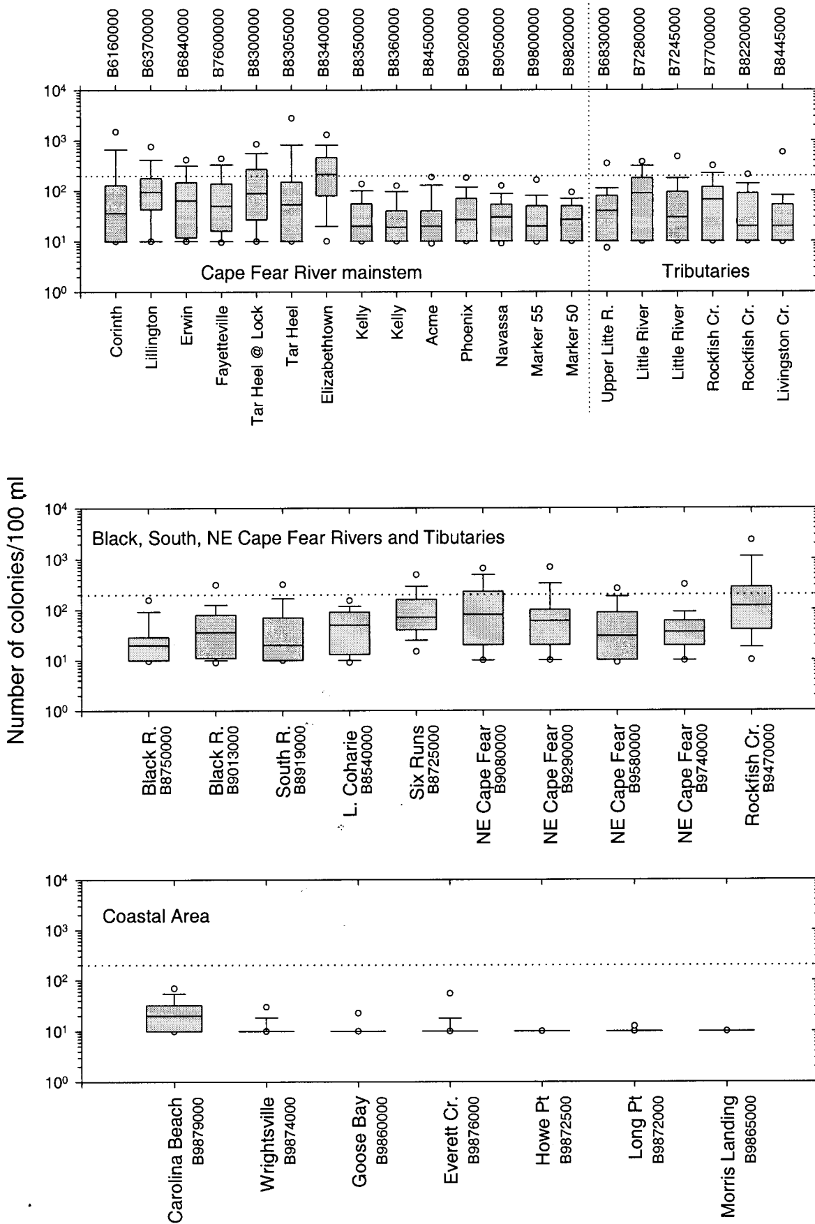
Figure A-17. Concentrations of fecal coliform bacteria (1993-1997). (Note the logarithmic scaling for the y-axis. A reference line representing 200 colonies per 100 milliliters is provided.)
