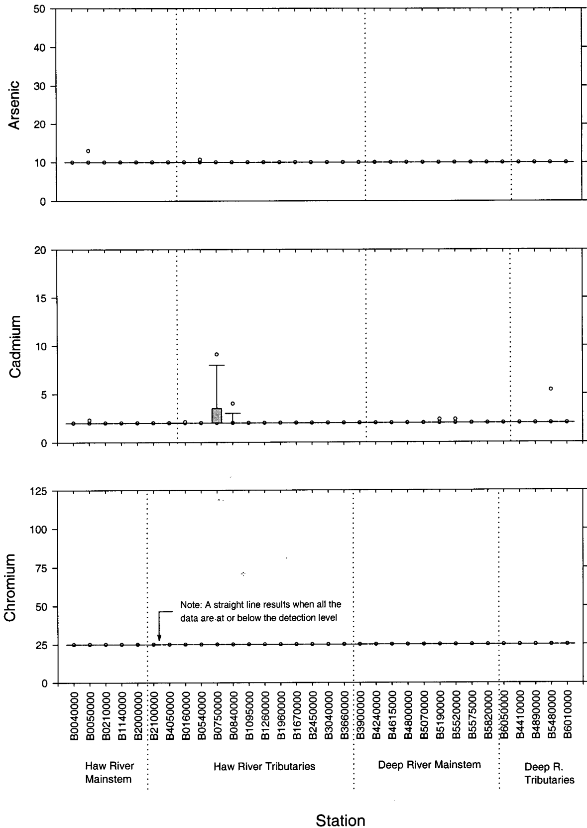
Figure A-18. Box plots of the concentrations ( \mu\text{g/l} ) of arsenic, cadmium and chromium for monitoring stations along the Haw and Deep rivers
