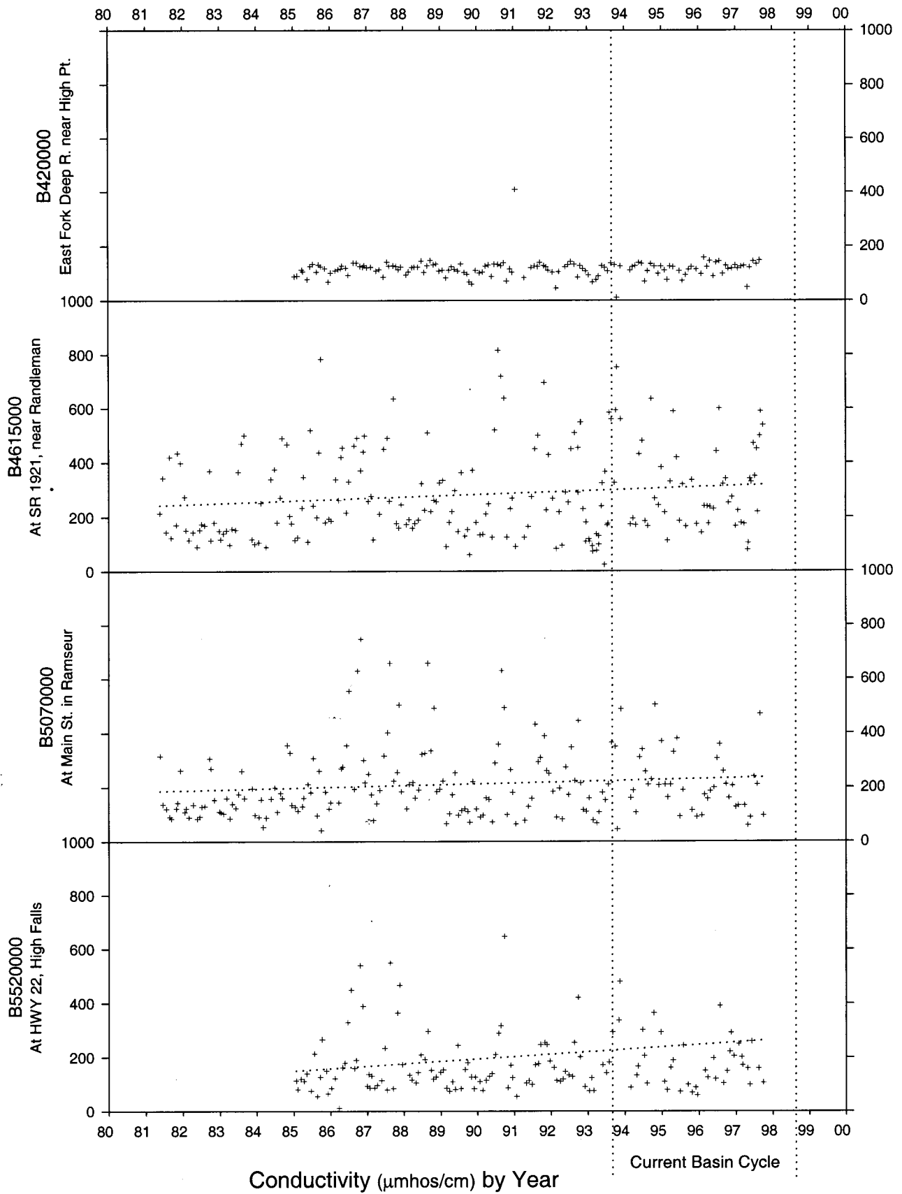
Figure A-32. Measurements of conductivity (y-axis) over time (x-axis) from four monitoring stations along the Deep River. (Stations are arranged in an upstream (top) - downstream (bottom) pattern.)
