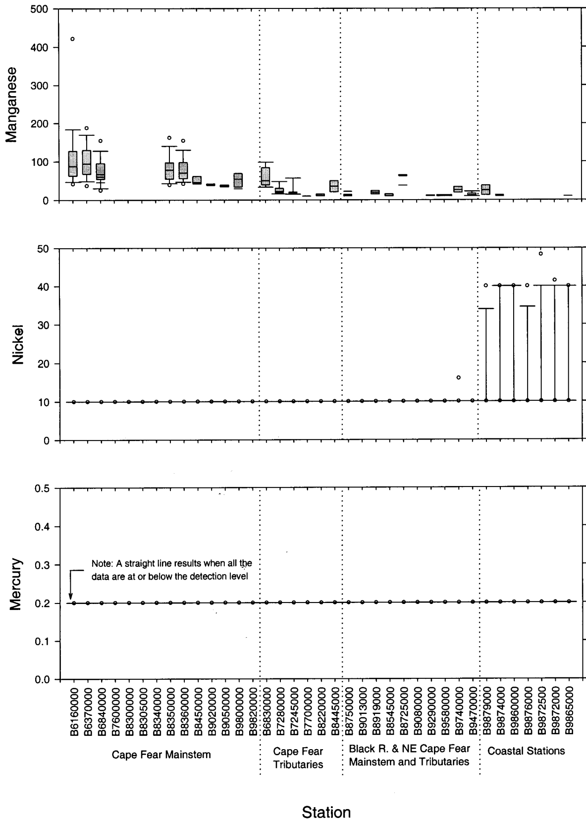
Figure A-23. Box plots of the concentrations ( \mu\text{g/l} ) of manganese, nickel and mercury for monitoring stations along the Cape Fear, Black, NE Cape Fear rivers, and along the coast.
