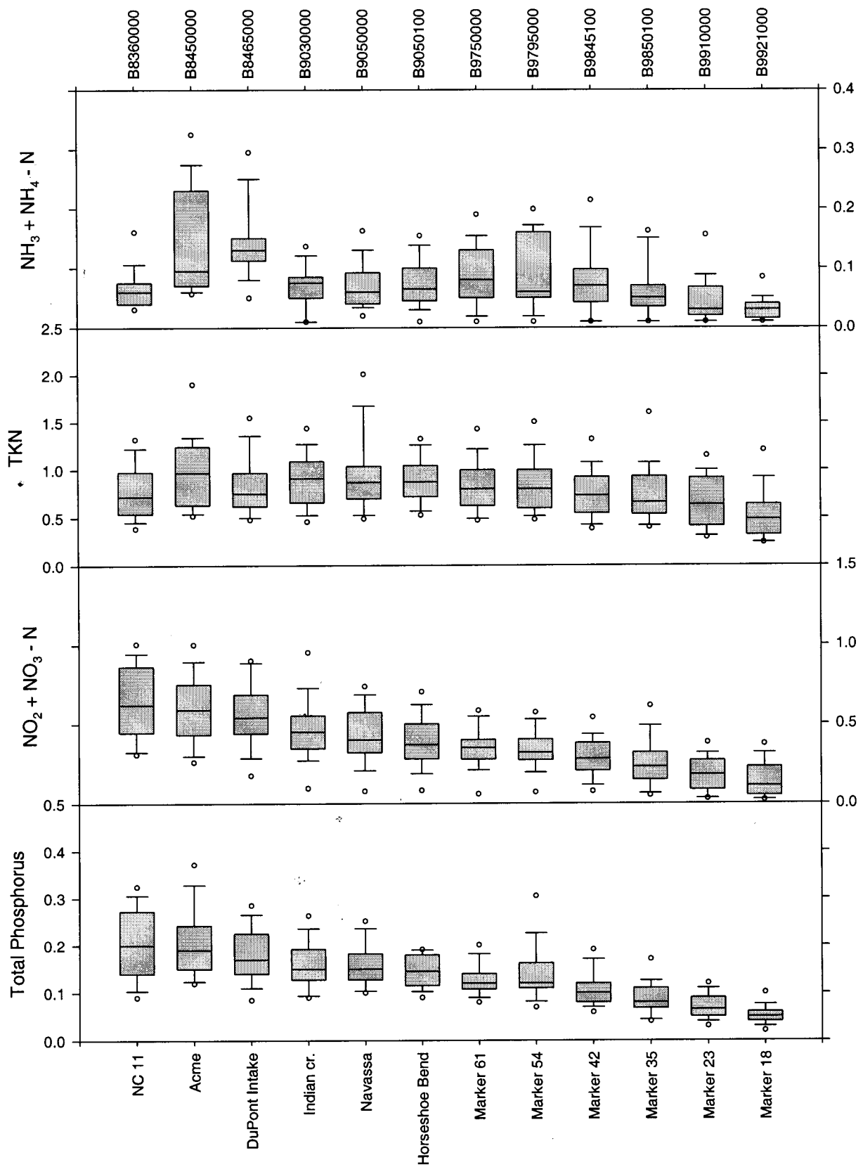
Figure A-47. Box plots for nutrients (mg/l) for the monitoring stations along the mainstem of the Cape Fear River. (Data were collected by the Lower Cape Fear River Program)
