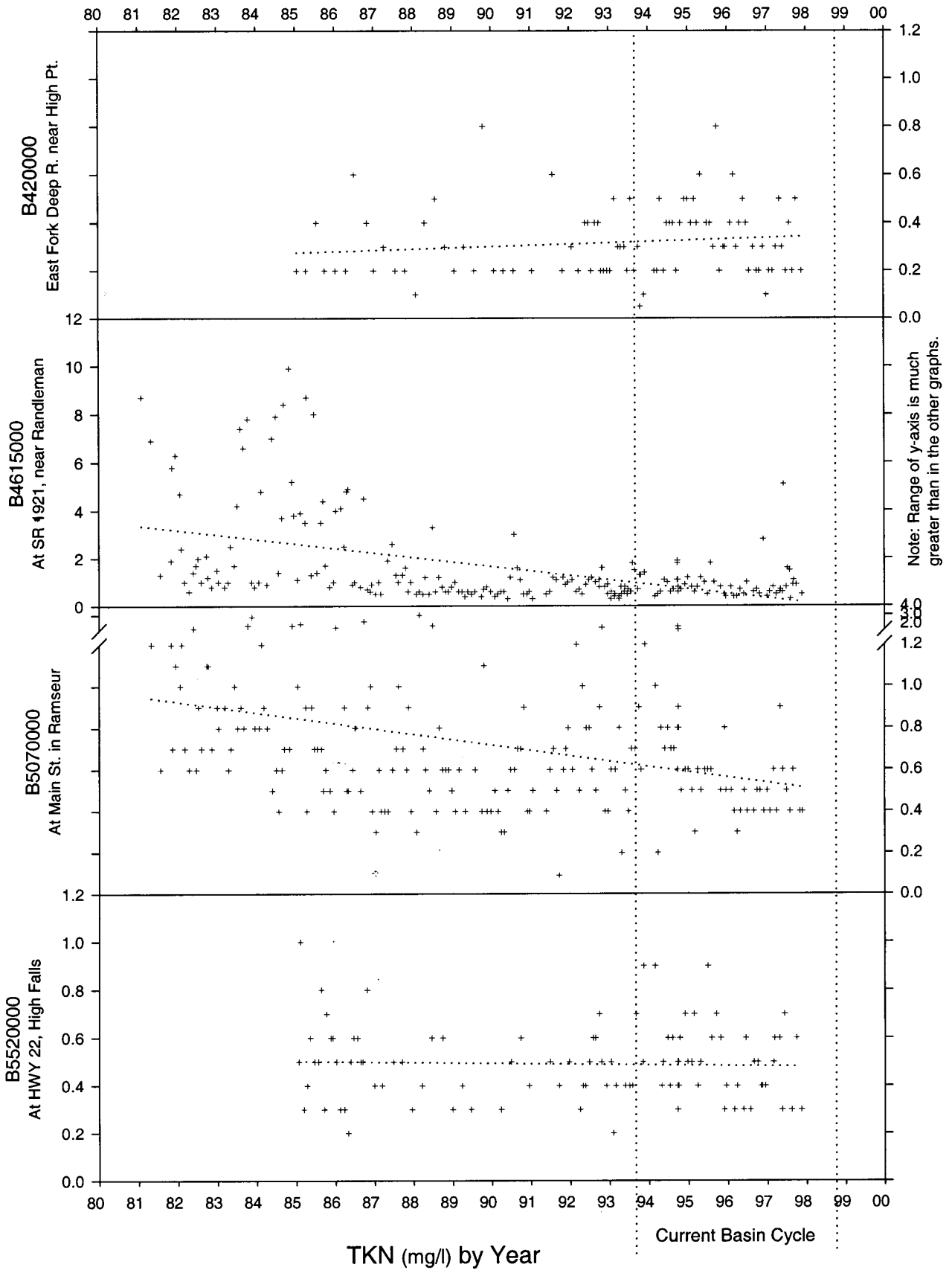
Figure A-35. Measurements of total Kjeldahl nitrogen (TKN; y-axis) over time (x-axis) from four monitoring stations along the Deep River. (Stations are arranged in an upstream (top) - downstream (bottom) pattern.)
