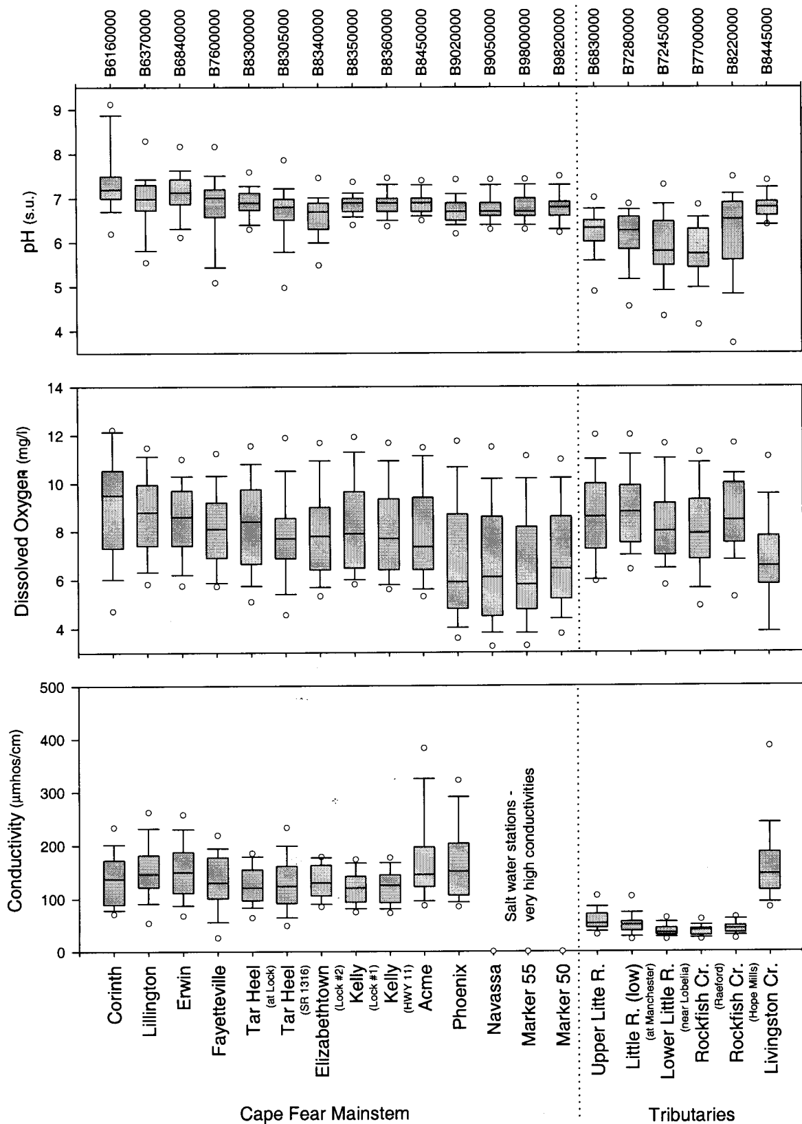
Figure A-8. Box plots for dissolved oxygen, pH and conductivity for the monitoring stations along the mainstem of the Cape Fear River (1993-1997).
