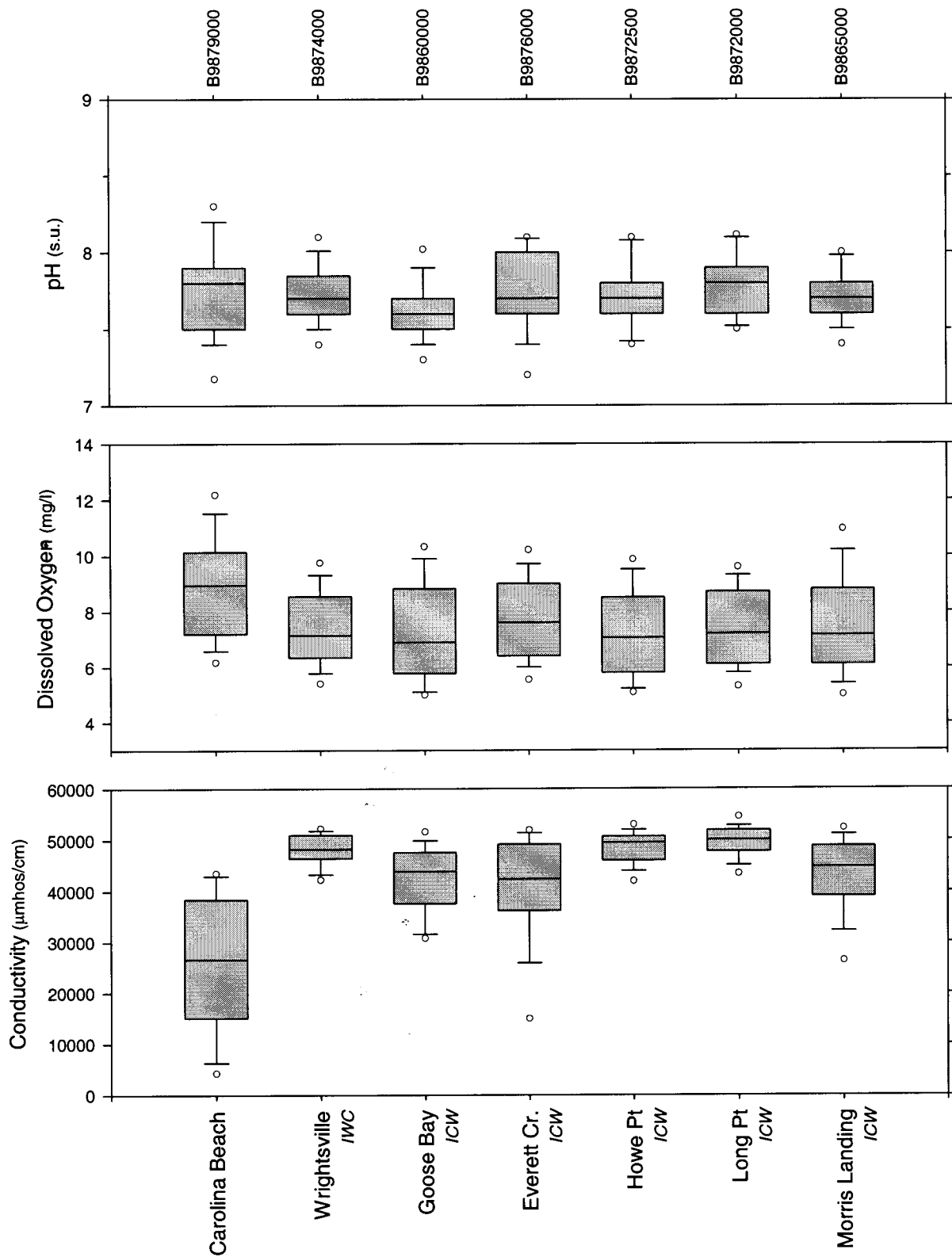
Figure A-14. Box plots for dissolved oxygen, pH and conductivity for seven monitoring stations along the coast (1993-1997). Note: Conductivity is not a useful parameter for interpreting water quality at saline stations. The data are presented here in order to be consistent with the other graphs.
