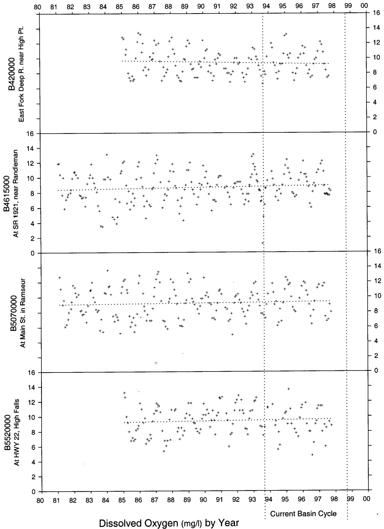
Figure A-33. Measurements of dissolved oxygen (y-axis) over time (x-axis) from four monitoring stations along the Deep River. (Stations are arranged in an upstream (top) - downstream (bottom) pattern.)
