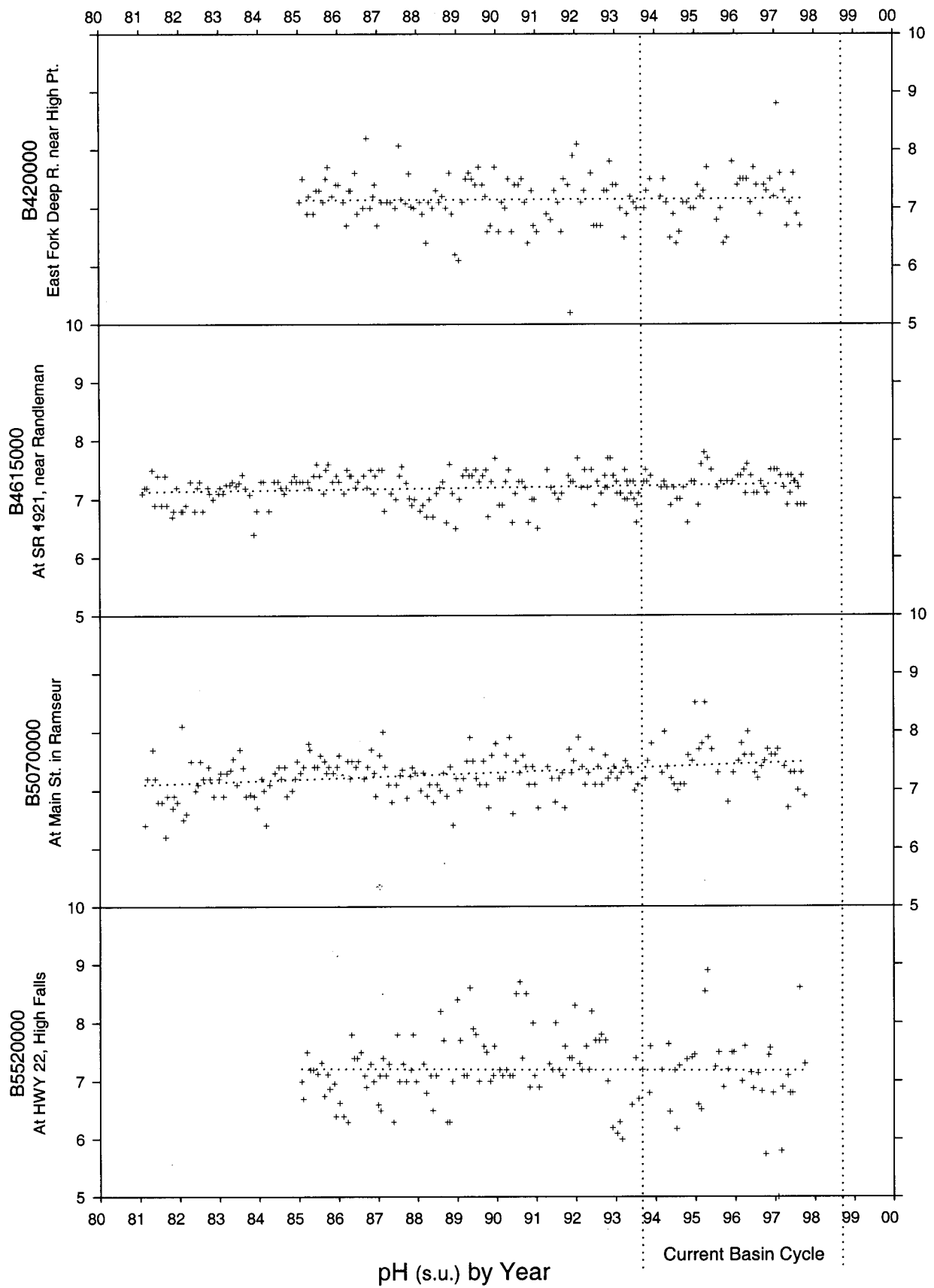
Figure A-31. Measurements of pH (y-axis) over time (x-axis) from four monitoring stations along the Deep River. (Stations are arranged in an upstream (top) - downstream (bottom) pattern.)
