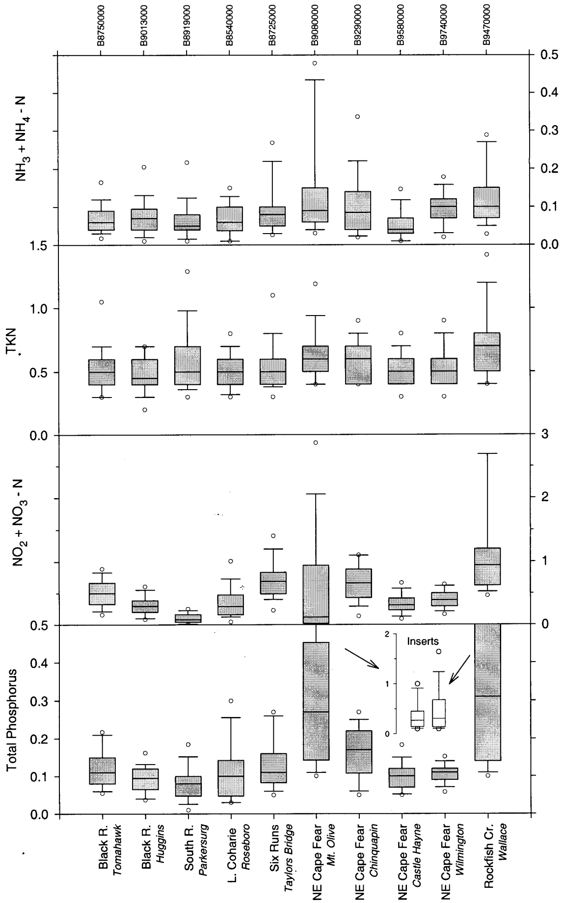
Figure A-11. Nutrients (mg/l) for the Black, South and NE Cape Fear Rivers and various tributaries (1993-1997; Insert represents expanded views of plots. Figure 13 provides the temporal patterns of these parameters for station B9080000 near Mt. Olive)
