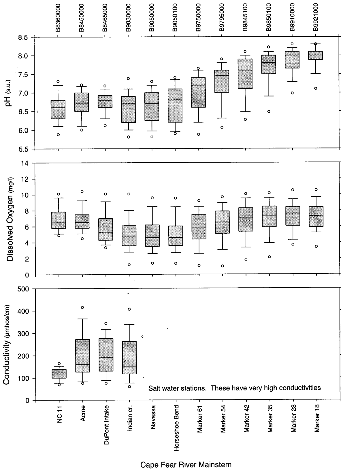
Figure A-45. Box plots for dissolved oxygen, pH and conductivity for the monitoring stations along the mainstem of the Cape Fear River (1996-1998). (Data were collected by the Lower Cape Fear River Program.)
