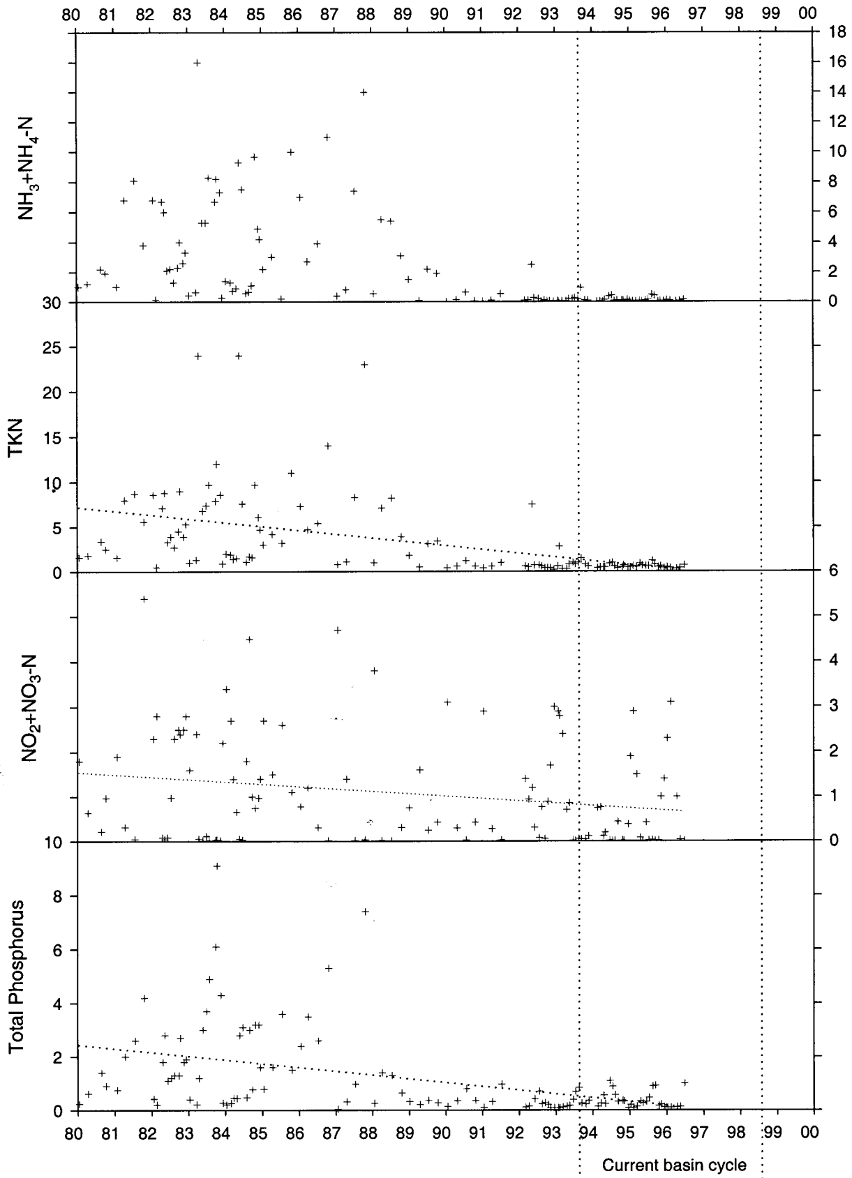
Figure A-13. Temporal patterns for nutrients (all mg/l) for station B9080000, NE Cape Fear at SR 1937 near Mt. Olive
