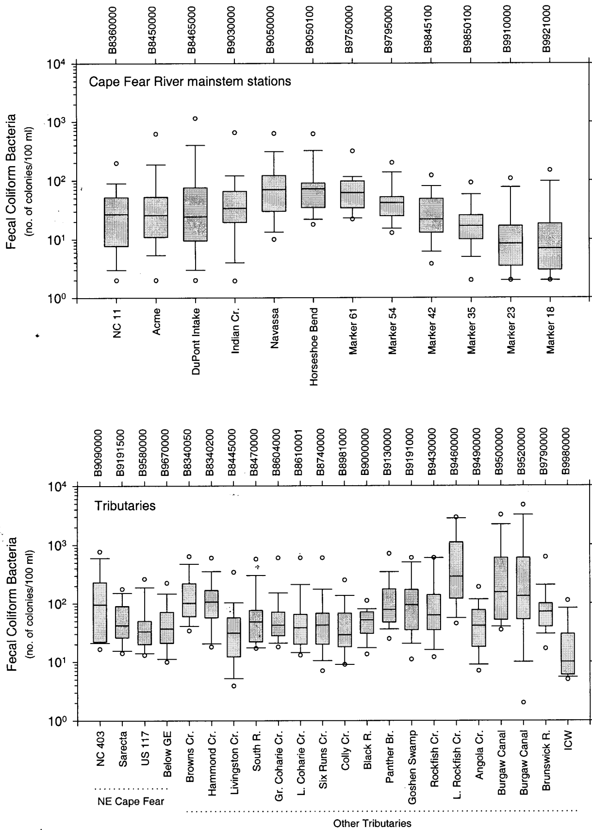
Figure A-49. Fecal Coliform measurements from stations along the Cape Fear River and tributaries (1996-1998). (Data were collected by the Lower Cape Fear River Program).
