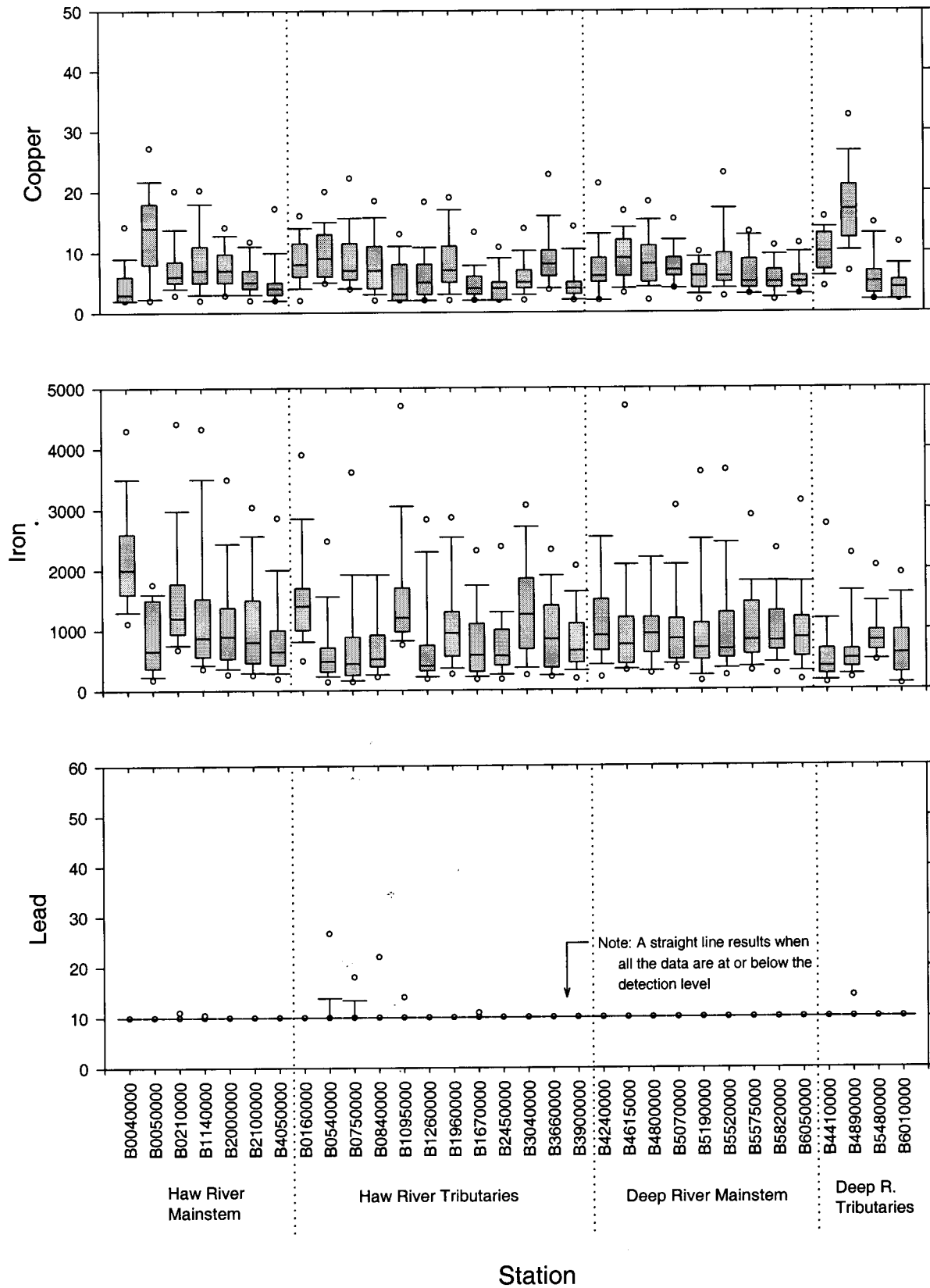
Figure A-20. Box plots of the concentrations ( \mu\text{g/l} ) of copper, iron and lead for monitoring stations along the Haw and Deep rivers.
