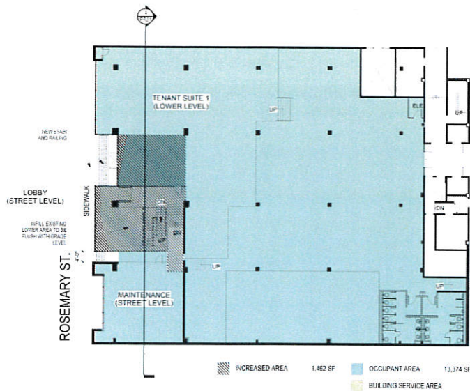
⑦ ROSEMARY LOWER LEVEL - DAY 2 1/16" = 1'-0"
