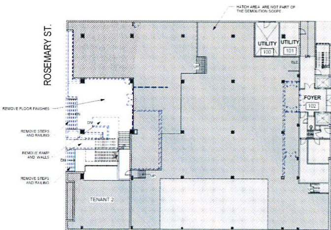
ROSEMARY LOWER LEVEL DEMOLITION PLAN 1/17' = 1" = 0'
