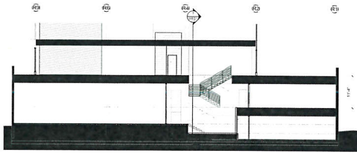
⑥ Section 18 3/32" = 1'-0"
