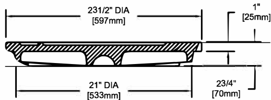
COVER SECTION
