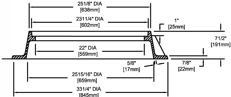
FRAME SECTION
