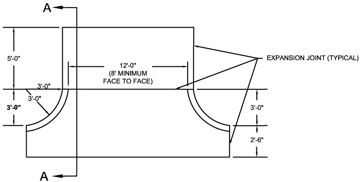
TYPICAL DRIVEWAY APRON
