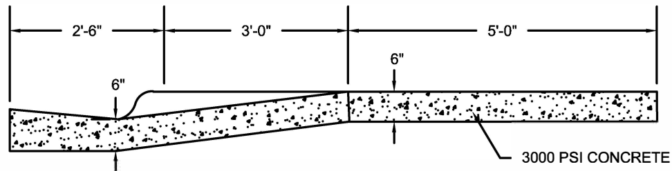
DRIVEWAY SECTION A-A
