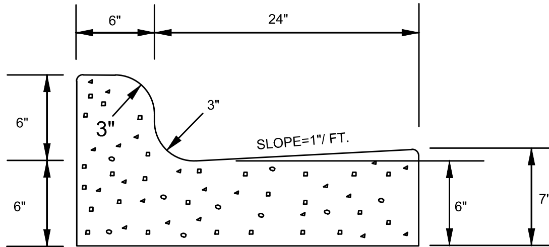
30" CURB & GUTTER
