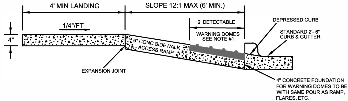
RAMP SECTION WITH DETECTABLE WARNING PAVERS
