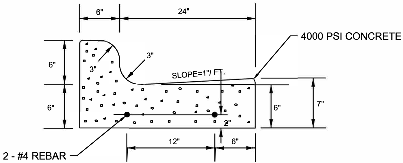
REINFORCED CURB AND GUTTER SECTION
