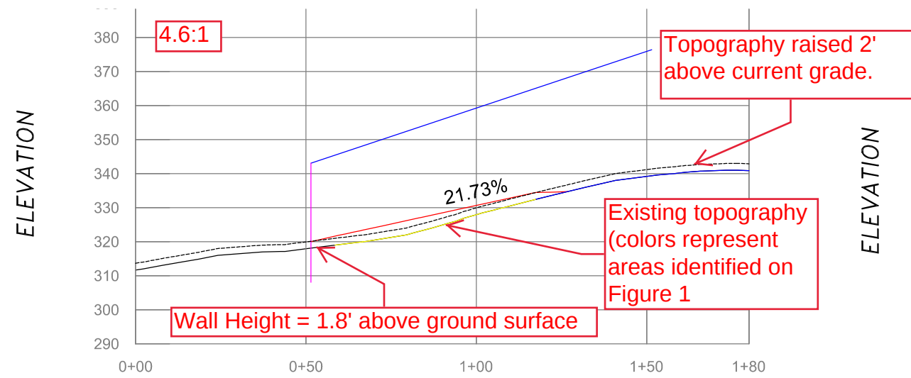
CROSS-SECTION "Alignment - A"
